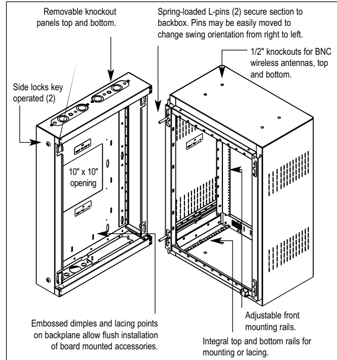
L250 BACKBOX
